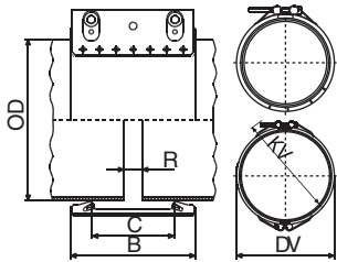
STRAUB-OPEN-FLEX 2 (2-piece execution shown)
