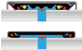
PROGRESSIVE SEALING EFFECT
