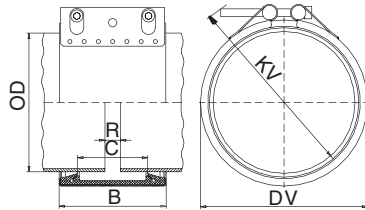
STRAUB-FLEX for Copper Tube
