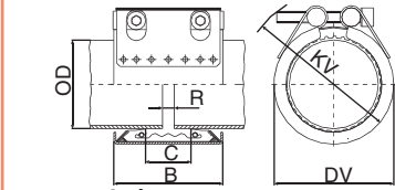
High-Pressure Type
