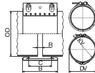
STRAUB-OPEN-FLEX for Copper Tube
